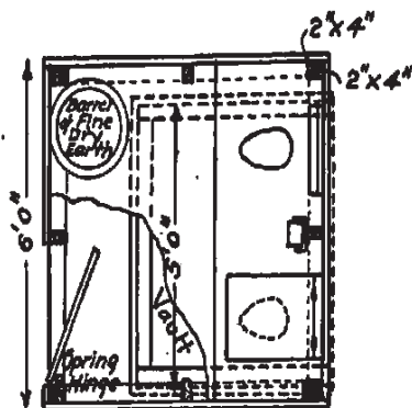
FIG. 1 PRIVY WITH VAULT
