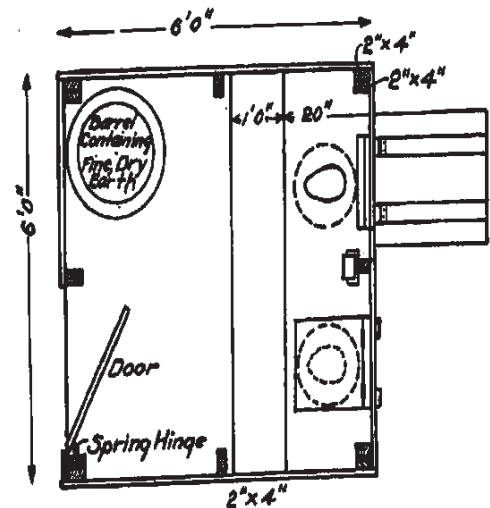
FIG. 2 PRIVY HAVING REMOVABLE CONTAINER
