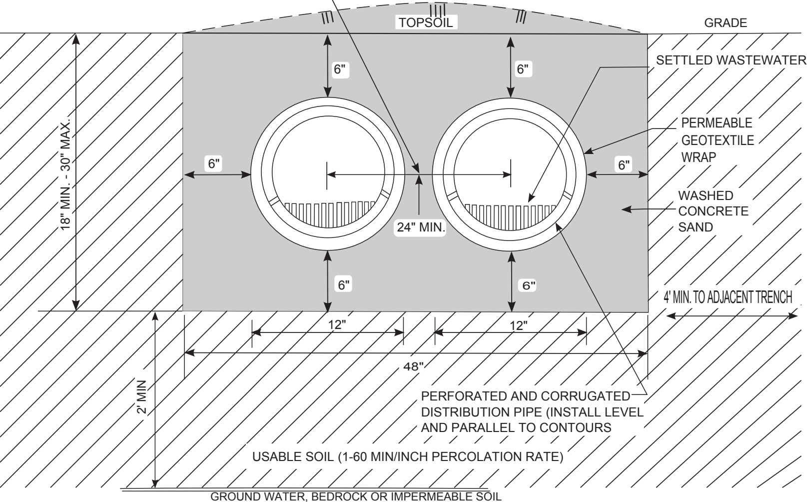
FIGURE 21: TYPICAL GRAVELLESS GEOTEXTILE SAND FILTER SYSTEMS
